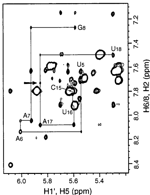
FIGURE 2: Base H6/8-to-H1' region of the 2D 160 ms NOESY spectrum. The sequential walk is traced through the bulge region (residues U 5 –G 8 and C 15 –U 18 ) with intraresidue peaks labeled. The arrow points to the long-range NOE between A 7 H 2 and A 17 H 1 '.
